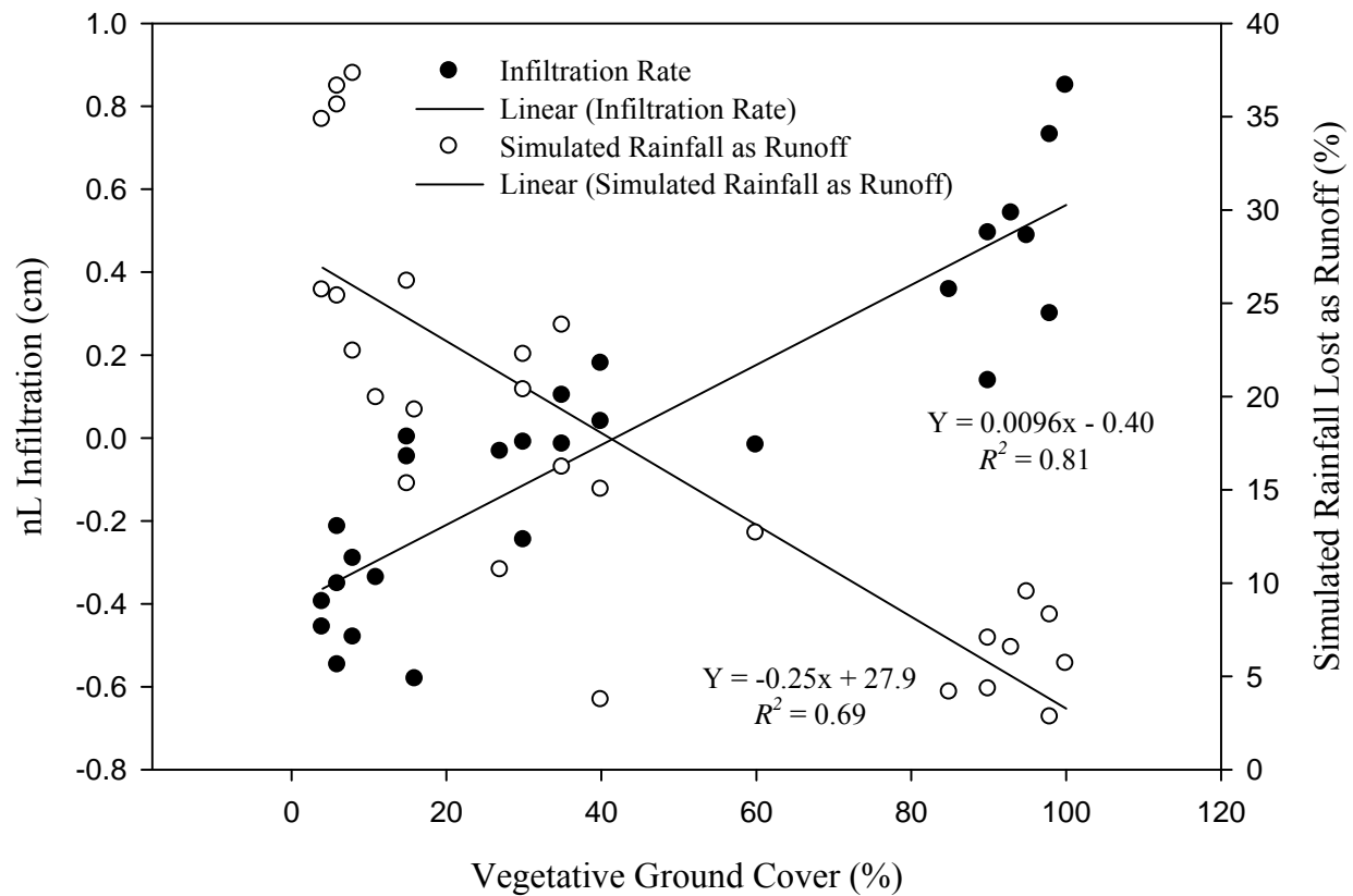
Figure 3.2. Soil infiltration and percent of simulated rainfall lost as runoff water as a function of percent vegetative ground cover. Significant at \alpha = 0.05 . Separate regression lines for individual treatments are not shown as slopes were not different ( \alpha = 0.05 ) (Tables 3.3 and 3.4).
