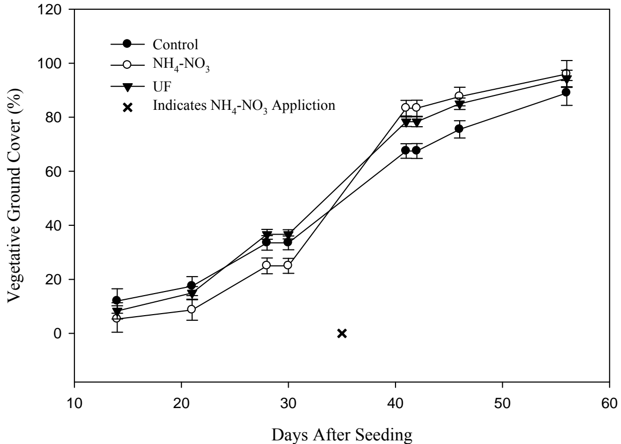
Figure 3.4. Bermudagrass vegetative ground cover as a function of time. Each point represents a mean of three replicates.
