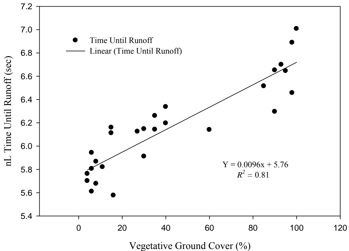
Figure 3.1. Time until runoff as a function of percent vegetative ground cover. Significant at \alpha = 0.05 . Separate regression lines for individual treatments are not shown as slopes were not different ( \alpha = 0.05 ) (Table 3.2 ).
