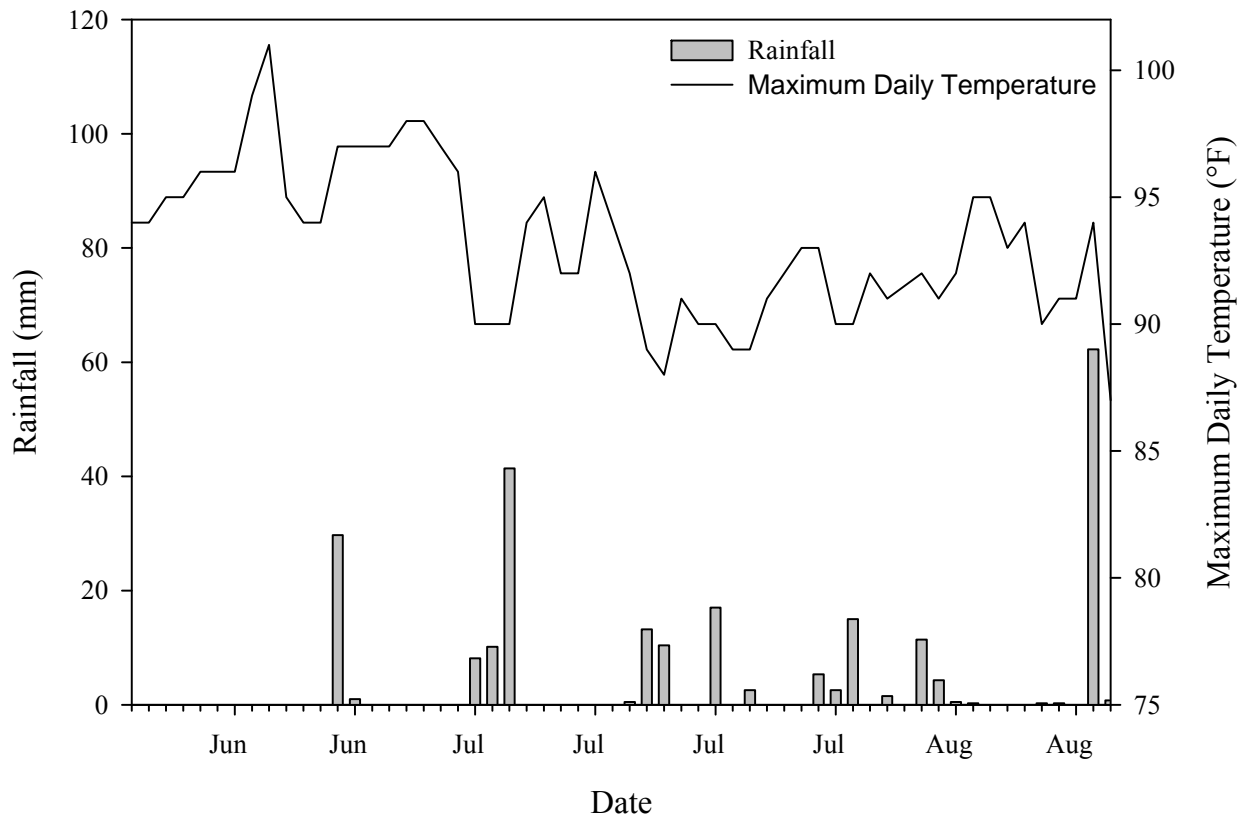
Figure A.2. Temperature and rainfall conditions of southeastern LA during summer 2009. Rainfall and maximum daily temperatures during summer 2009 runoff monitoring period. Data recorded 12.2 miles from research levee at the New Orleans International Airport.
