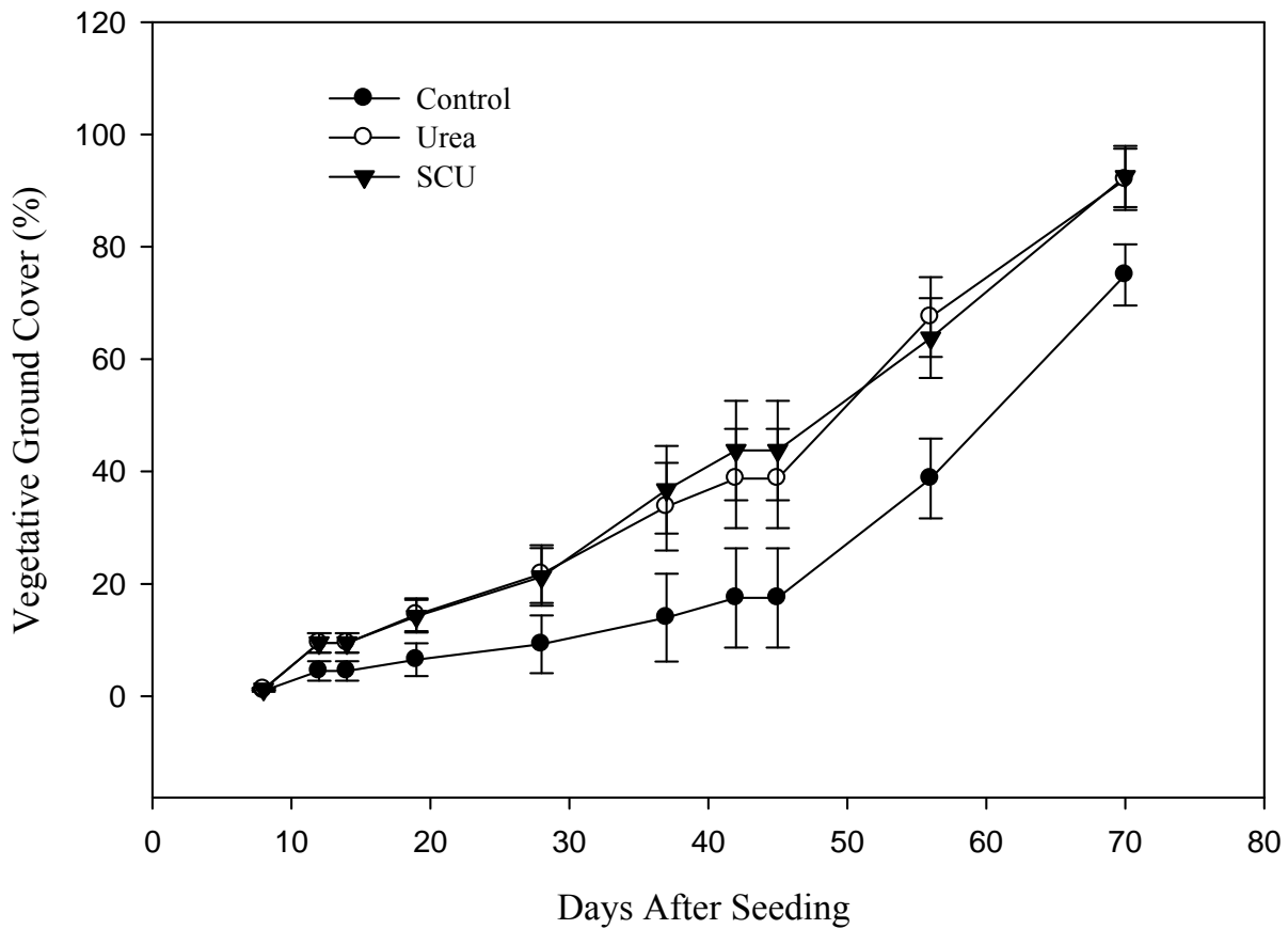
Figure 2.4. Bermudagrass vegetative ground cover as a function of time. Each point represents a mean of four replicates.
