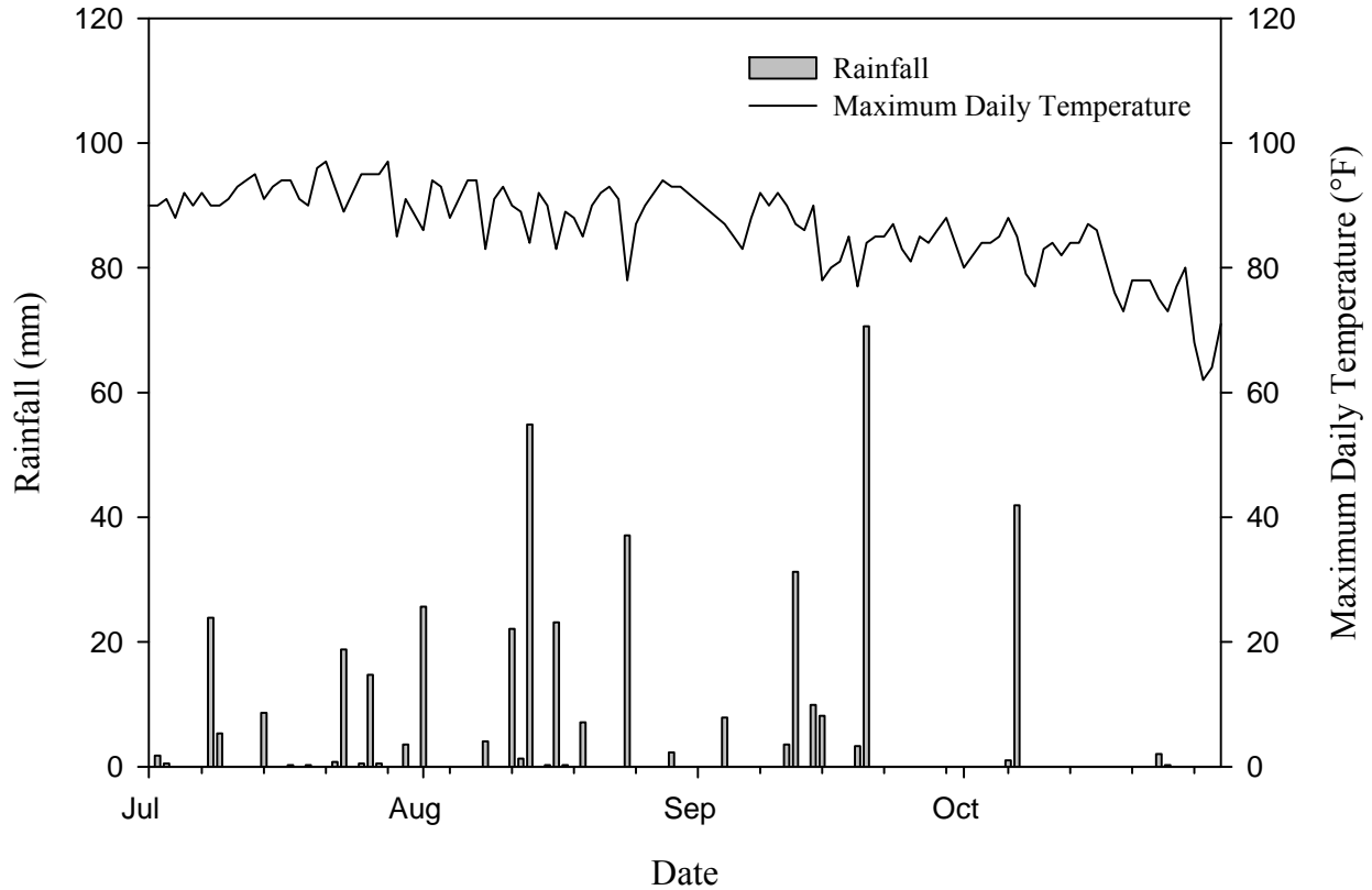
Figure A.1. Temperature and rainfall conditions of southeastern LA during summer 2008. Rainfall and maximum daily temperatures during summer 2008 runoff monitoring period. Data recorded 12.2 miles from research levee at the New Orleans International Airport.
