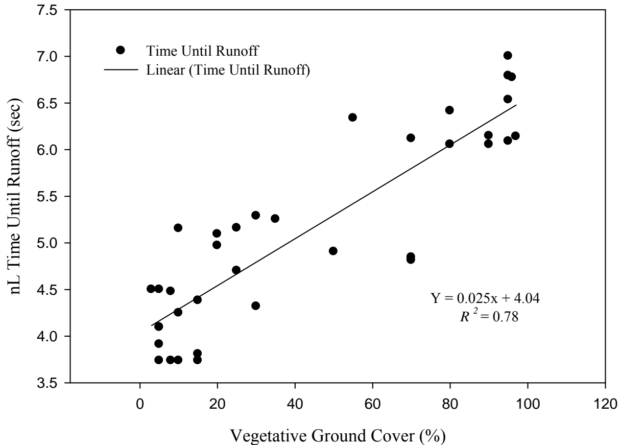
Figure 2.1. Time until runoff as a function of percent vegetative ground cover. Significant at \alpha = 0.05 . Separate regression lines for individual treatments are not shown as slopes were not different ( \alpha = 0.05 ) (Table 2.2).
