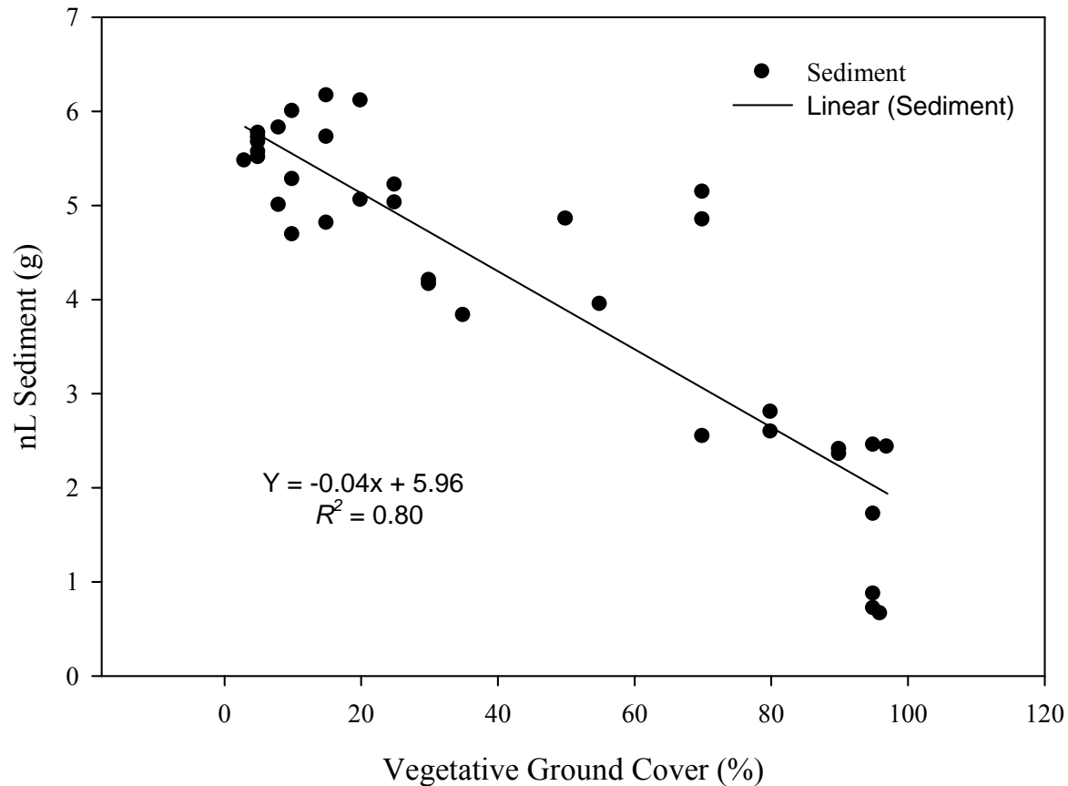
Figure 2.3. Sediment loss as a function of percent vegetative ground cover. Significant at \alpha = 0.05 . Separate regression lines for individual treatments are not shown as slopes were not different ( \alpha = 0.05 ) (Table 2.6).
