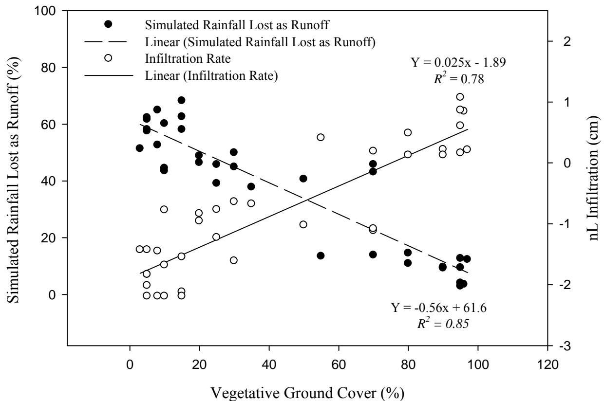
Figure 2.2. Soil infiltration and percent of simulated rainfall lost as runoff water as a function of percent vegetative ground cover. Significant at \alpha = 0.05 . Separate regression lines for individual treatments are not shown as slopes were not different ( \alpha = 0.05 ) (Tables 2.3 and 2.4).
