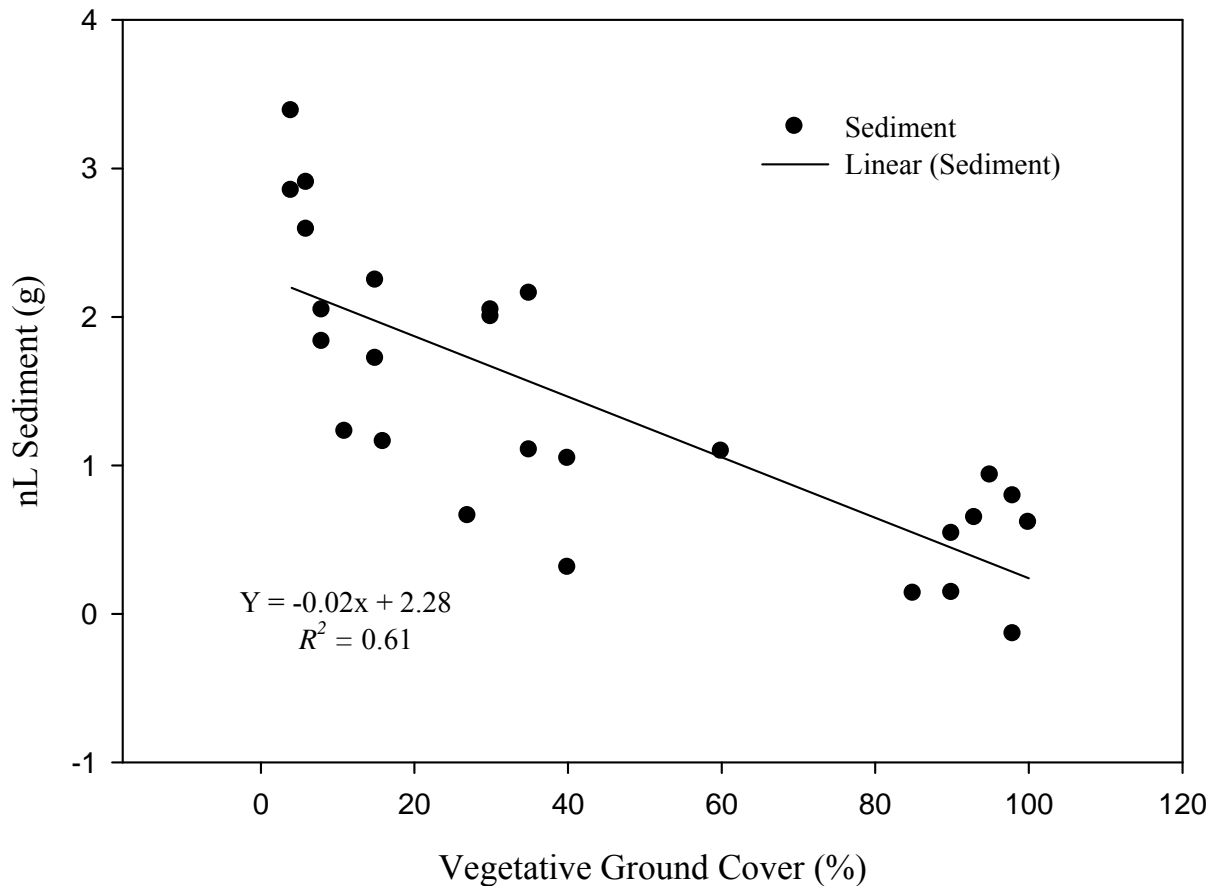
Figure 3.3. Sediment loss as a function of percent vegetative ground cover. Significant at \alpha = 0.05 . Separate regression lines for individual treatments are not shown as slopes were not different ( \alpha = 0.05 ) (Table 3.6).
