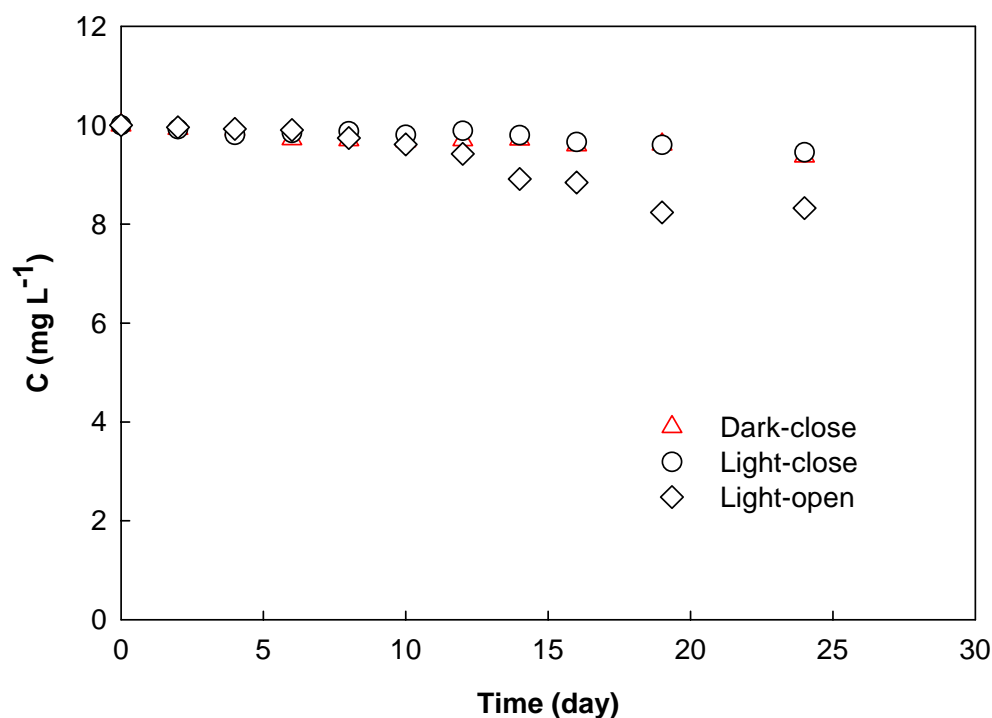
Fig. 2.3. Tylosin stability under dark and light conditions in H 2 O. Tylosin solutions (10mg L -1 ) were incubated in dark with vial cap closed (dark-close), light with vial cap closed (light-close) and light with vial cap opened (light-open) for times shown at 25 °C.
