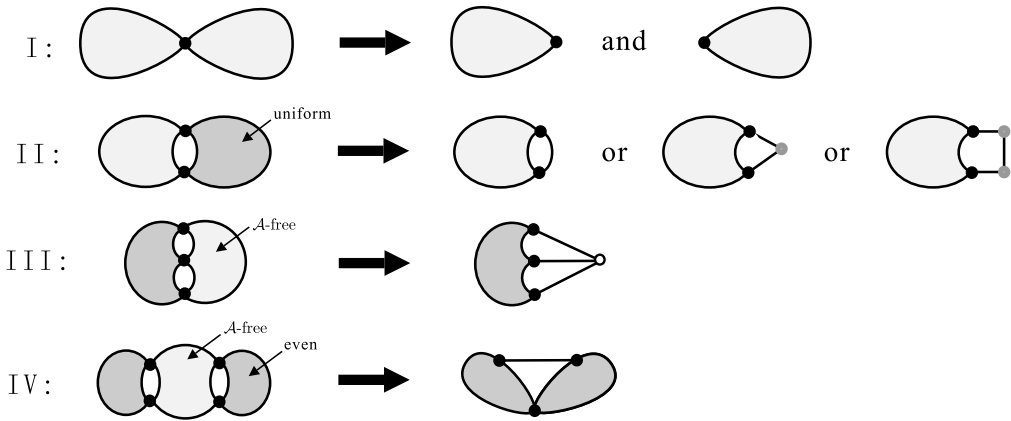
Fig. 1. Reductions I, II, III, and IV.
