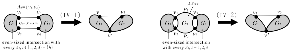
Fig. 3. Reduction IV based on even 4-separation (G_1 \cup G_2, G_3) at \{v_1, v_2, v_3, v_4\} .
