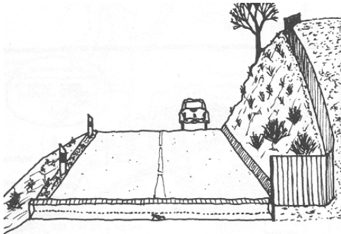
Fig. 3.7: Amphibian tunnel under roadway with drift fencing. (From Dramstad, Landscape Ecology Principles in Landscape Architecture and Land-Use Planning , 62)
