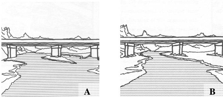
Fig. 3.8: A illustrates the wrong way to design a wildlife overpass: there is no dry land crossing underneath the span. B illustrates the correct way to design a wildlife overpass, where there is dry land on either side of the waterway. (From Dramstad, Landscape Ecology Principles in Landscape Architecture and Land-Use Planning , 55)
