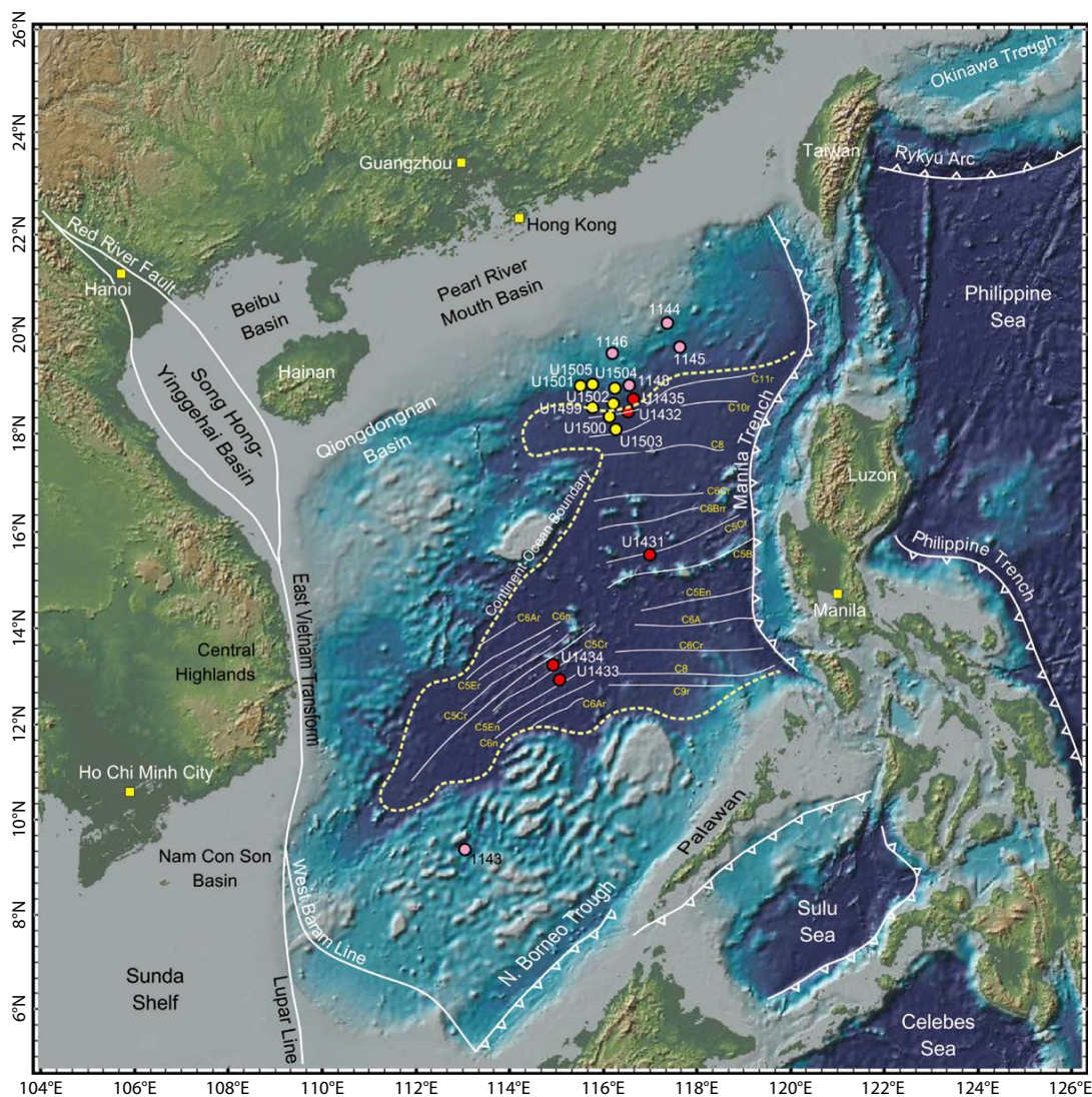
FIGURE 1. Regional geodynamic framework of the South China Sea. Circles mark the drill sites of Ocean Drilling Program Leg 184 (pink), International Ocean Discovery Program (IODP) Expedition 349 (red), and IODP Expeditions 367, 368, and 368X (yellow). The yellow dotted line around the basin marks the continent-ocean boundary. Magnetic isochrons are based on C.F. Li et al. (2014).
