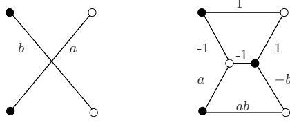
FIGURE 8. Replace crossing edges with the butterfly.
