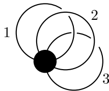
Figure 31: We compute the Khovanov homology Kh(\mathbb{G}) and reduced Khovanov homology \widetilde{Kh}(\mathbb{G}) for the depicted ribbon graph \mathbb{G} .
