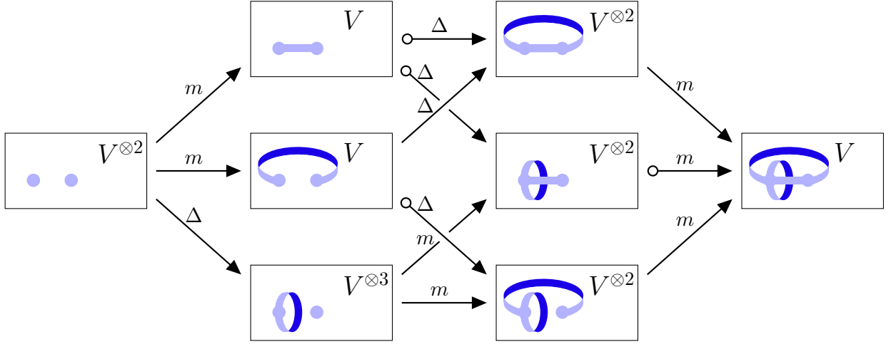
Figure 5: The set of ribbon subgraphs arranged into a hypercube. Each vertex \mathbb{G}(I) is labeled with V^{\otimes F(\mathbb{G}(I))} . The edges of the cube are labeled according either m or \Delta corresponding to a merge or a split of boundary components respectively. If the sign of an edge map is negative, then there is a small circle on the tail of the edge.
