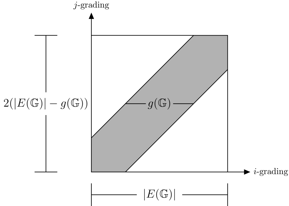
Figure 30: For a ribbon graph \mathbb{G} , the reduced Khovanov homology \widetilde{Kh}(\mathbb{G}) can only be nontrivial within the shaded region.
