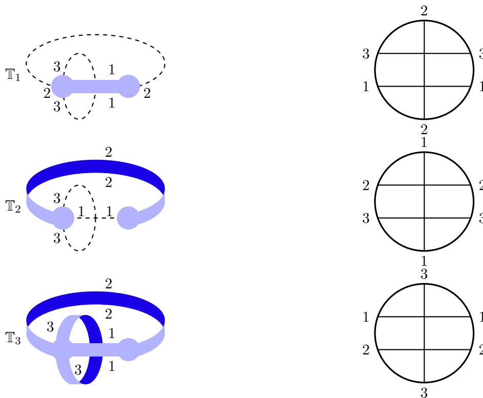
Figure 25: The three spanning quasi-trees \mathbb{T}_1 , \mathbb{T}_2 , and \mathbb{T}_3 of \mathbb{G} and their corresponding chord diagrams.
