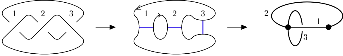
Figure 7: To construct the all- A ribbon graph, first construct the all- A Kauffman state. Then the components of the all- A Kauffman state become the vertices, and the traces of the crossings become the edges.
