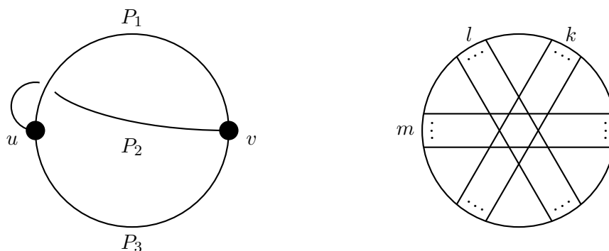
Figure 27: Left: A schematic depiction of the first type of a ribbon subgraph of \mathbb{T} . Right: The corresponding configuration in the chord diagram C(\mathbb{G}, \mathbb{T}) .
