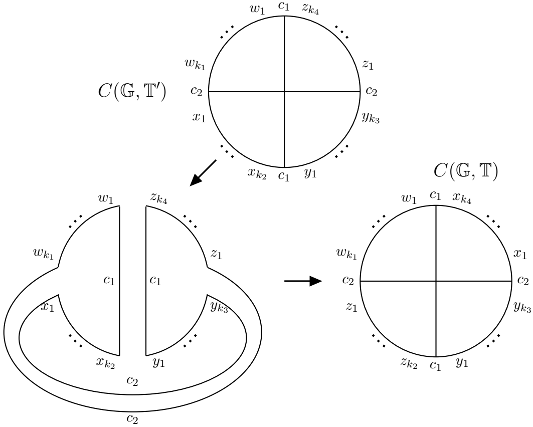
Figure 29: Chords c_1 and c_2 are exterior in C(\mathbb{G}, \mathbb{T}') . Surgering bands along c_1 and c_2 results in a one component diagram, which can be smoothly deformed to give the chord diagram C(\mathbb{G}, \mathbb{T}) , where c_1 and c_2 are interior.
