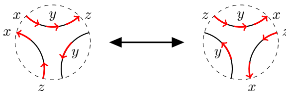
Figure 18: A Reidemeister III move on an arrow presentation.
