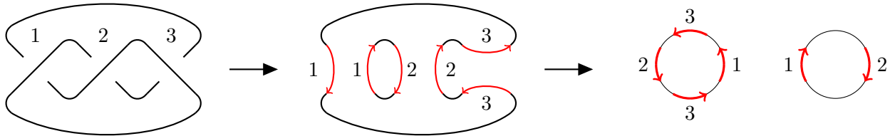
Figure 9: The construction of the arrow presentation for the all- A ribbon graph of a link diagram D .
