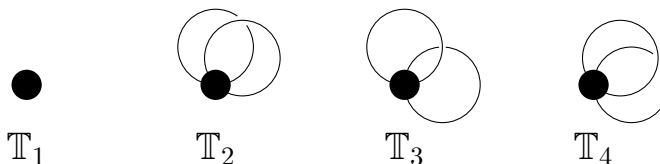
Figure 33: The four spanning quasi-trees of \mathbb{G} .
