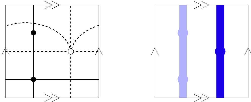
Figure 2: Left: The ribbon graph \mathbb{G} is depicted with black vertices and solid edges, while the ribbon graph \mathbb{G}^* is depicted with white vertices and dashed edges. Right: Ribbon subgraphs \mathbb{H} and \widehat{\mathbb{H}} of \mathbb{G} and \mathbb{G}^* respectively.
