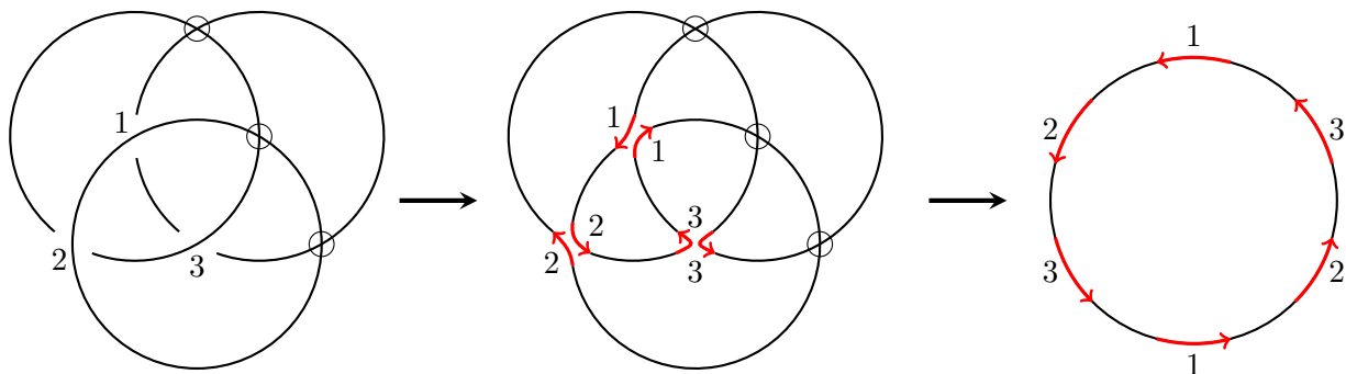
Figure 14: Transforming a virtual link diagram D into an arrow presentation P(D) .
