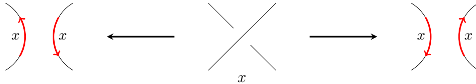
Figure 8: The A -resolution of a crossing labeled by x with the two equivalent choices of orientations of marking arrows.
