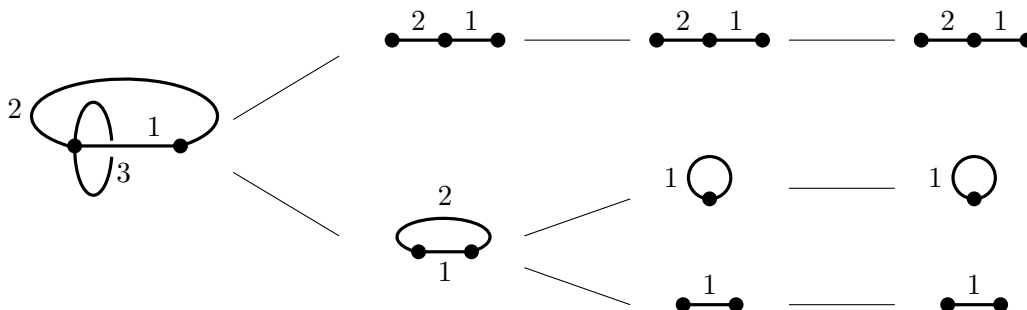
Figure 23: The tree \mathcal{J}(\mathbb{G}) for the ribbon graph of Figure 1.
