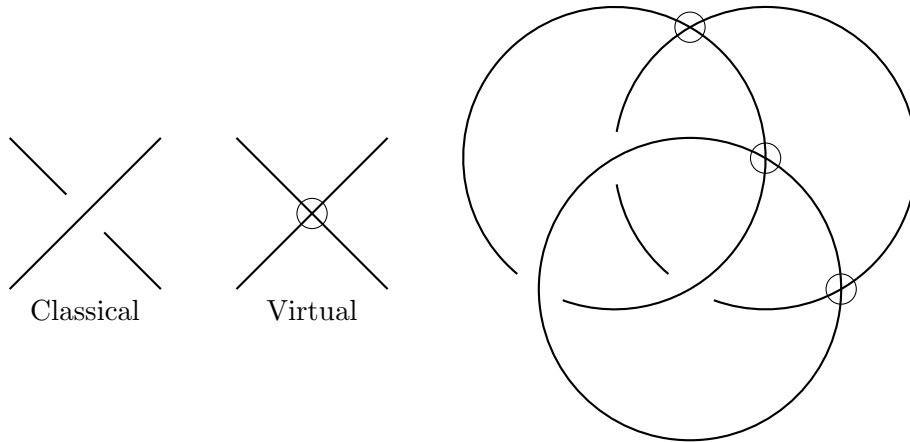
Figure 11: A classical crossing, a virtual crossing, and a virtual link diagram
