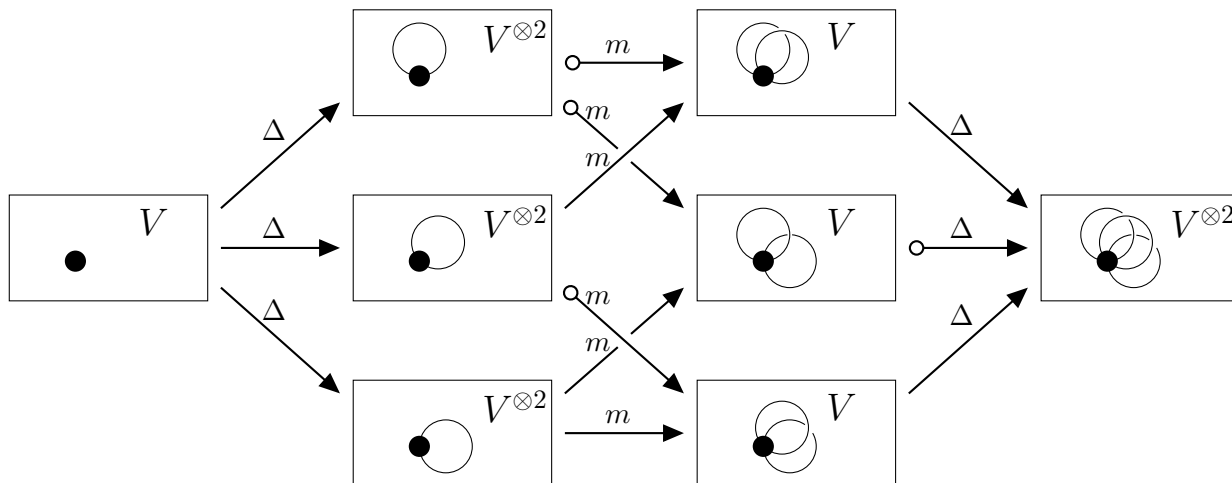
Figure 32: The hypercube complex for the ribbon graph \mathbb{G} in Figure 31.
