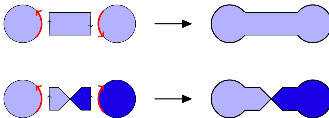
Figure 3: Attaching bands to pairs of identically labeled marking arrows.
