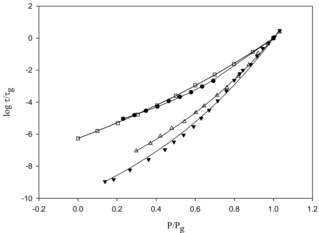
Figure 7 Plot of the log of scaled dielectric relaxation time versus scaled pressure for PMTS ( \square ), PPG ( \triangle ), DGEB ( \bullet ) and DEP ( \blacktriangledown ) at \sim 293 K. Model fits are shown as lines with parameters of Table 1 and experimental data 27,25,92,93 as points. The defined point at \log \tau_i^*/\tau_g = 0 at P/P_g = 1 has been added to the data sets.
