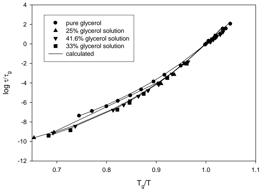
Figure 28 Plot of temperature dependence of relaxation time showing experimental data for pure glycerol (●), glycerol relaxation in 25 wt% aqueous glycerol solution (▲), glycerol relaxation in 33 wt% aqueous glycerol solution (■), and glycerol relaxation in 41.6 wt% aqueous glycerol solution (▼). Lines are fits of experimental data for pure glycerol, and calculated dielectric relaxation times for solutions.
