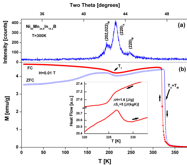
FIG. 1. (a) XRD pattern of \text{Ni}_{50}\text{Mn}_{34.8}\text{In}_{14.2}\text{B} obtained at 300 K using \text{CuK}\alpha radiation. Indexes “A” and “M” identify the XRD peaks from the cubic austenitic and tetragonal martensitic phases, respectively; (b) the temperature dependencies of the magnetization obtained at 0.01 T after the sample was cooled from 380 to 5 K at zero field (ZFC), and after cooling in the presence of a FC. Arrows indicate the transition temperatures. Inset: temperature dependencies of the heat flow of \text{Ni}_{50}\text{Mn}_{35}\text{In}_{14}\text{B} . Arrows indicate the direction of temperature changes.
